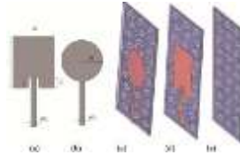
Fig.3. (a) rectangular patch, (b) circular patch, (c) circular patch with a CSRR array in the ground plane, and (d) rectangular patch antenna with a CSRR array in the ground plane (GP), and (e) superstrate with a CSSR array.
