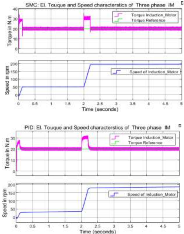
Figure 16. Electromagnetic torque and speed at load ( T=15\text{Nm} )
