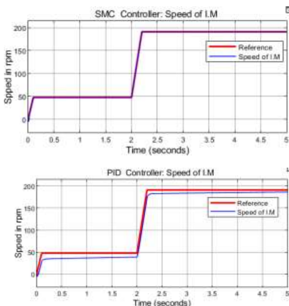
Figure 15. Speed of induction motor at load( T=15\text{Nm} )
