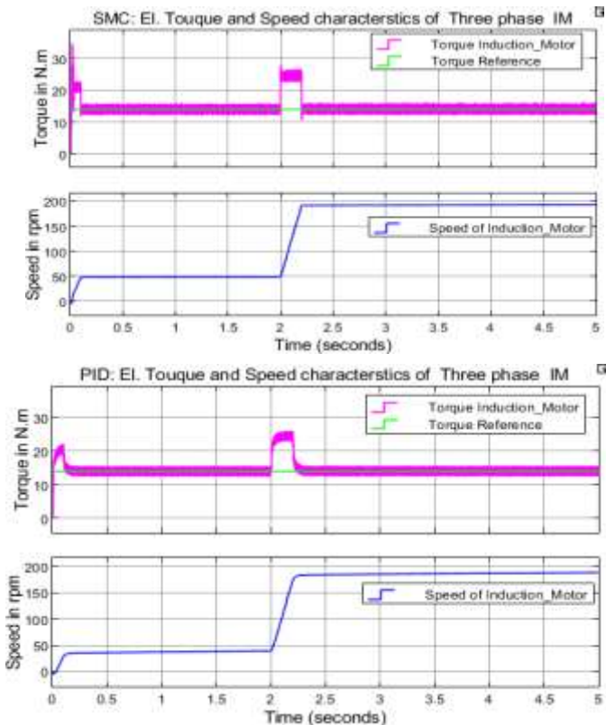
Figure14. Electromagnetic torque and speed at load ( T=15\text{Nm} )
