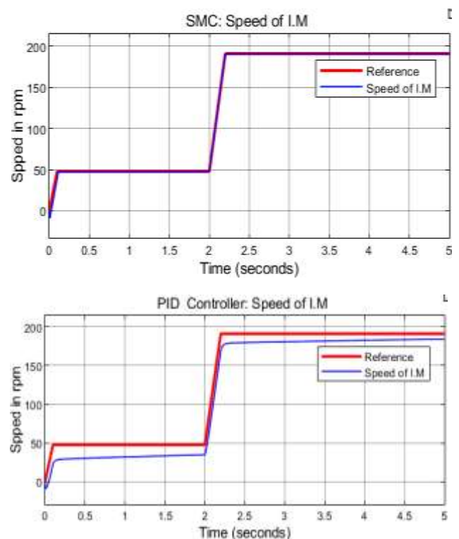
Figure 17. Speed of induction motor at load( T=20\text{Nm} )
