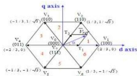
Figure 5. switching vectors and sectors
