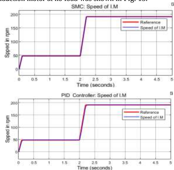
Figure 13. Speed of induction motor at no load( T=0\text{Nm} )
