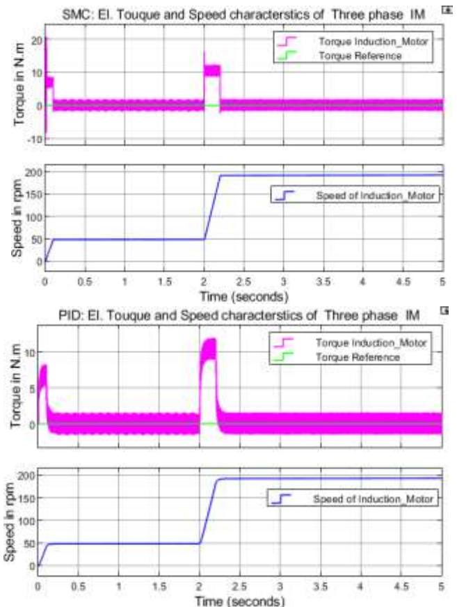
Figure 12. Electromagnetic torque and speed at no load( T=0\text{Nm} )
