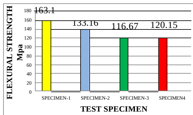
Fig 12 Results of Flexural Test
