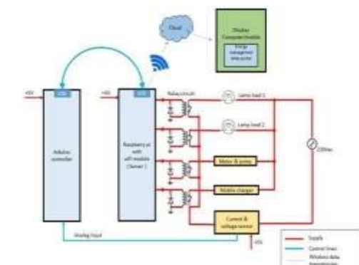
Figure 2 Circuit diagram of energy management module.
