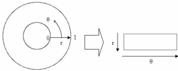
Figure 3.1 – Daugman's rubber sheet model.
