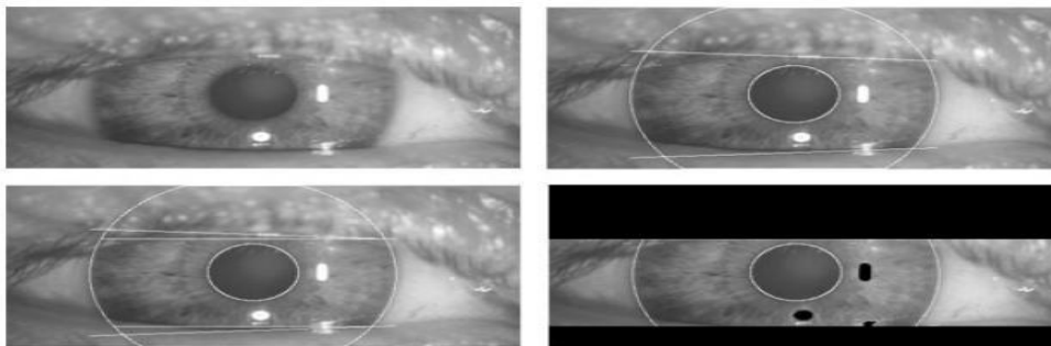
Figure 2.2 - Stages of division with eye picture "pi201b" from the LEI database Top left) unique eye picture Top right) two circles overlayed for iris and understudy limits, and two lines for top and base eyelid Bottom left) flat lines are drawn for every eyelid from the most minimal/most noteworthy purpose of the fitted line Bottom right) plausible eyelid and specular reflection regions disengaged (darkzones)
