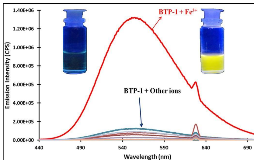
Fig. 3. Fluorescence emission change of sensor BTP-1 (2 mL, 2 \times 10^{-5} M, \text{CH}_3\text{CN} ) upon the addition of a particular metal ions (20 \mu\text{L} , 1 \times 10^{-2} M, in \text{H}_2\text{O} ), \lambda_{\text{ex}} = 314 nm.
