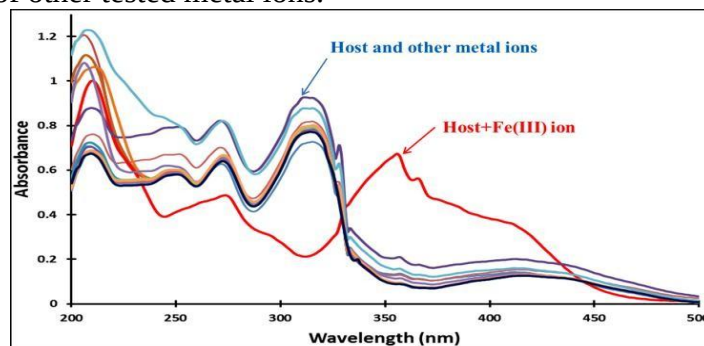
Fig. 1. Changes in the absorbance of BTP-1 (2 mL, 2 \times 10^{-5} M, in \text{CH}_3\text{CN} ) in absence and presence of 5 equivalents of different metal ions (20 \mu\text{L} , 1 \times 10^{-2} M, in \text{H}_2\text{O} ).
