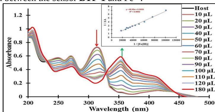
Fig. 2. Absorbance titration of BTP-1 ( 2 \times 10^{-5} M, in \text{CH}_3\text{CN} ) upon the addition of incremental amount of \text{Fe}^{3+} (0-180 \mu\text{L} , 1 \times 10^{-3} M, in \text{H}_2\text{O} ). Inset showing the Benesi-Hildebrand plot.
