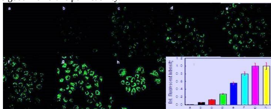
Fig. 6. Fluorescence confocal microscopic images of living HL-7701 cells incubated with various concentrations of \text{Fe}^{3+} . (a) Cells loaded with 50 \mu\text{M} of iron chelator desferoxamine (DFO) for 40 min. (b) Cells loaded with 10 \mu\text{M} BTP-1 for 10 min as control. (c) - (h) Cells incubated with 0.01, 0.1, 1, 10, 100 and 1000 \mu\text{M} \text{Fe}^{3+} , respectively. (i) Quantification of mean fluorescence intensity in Fig. S20a-S20h correspondingly. Scale bar is 20 \mu\text{m} .
