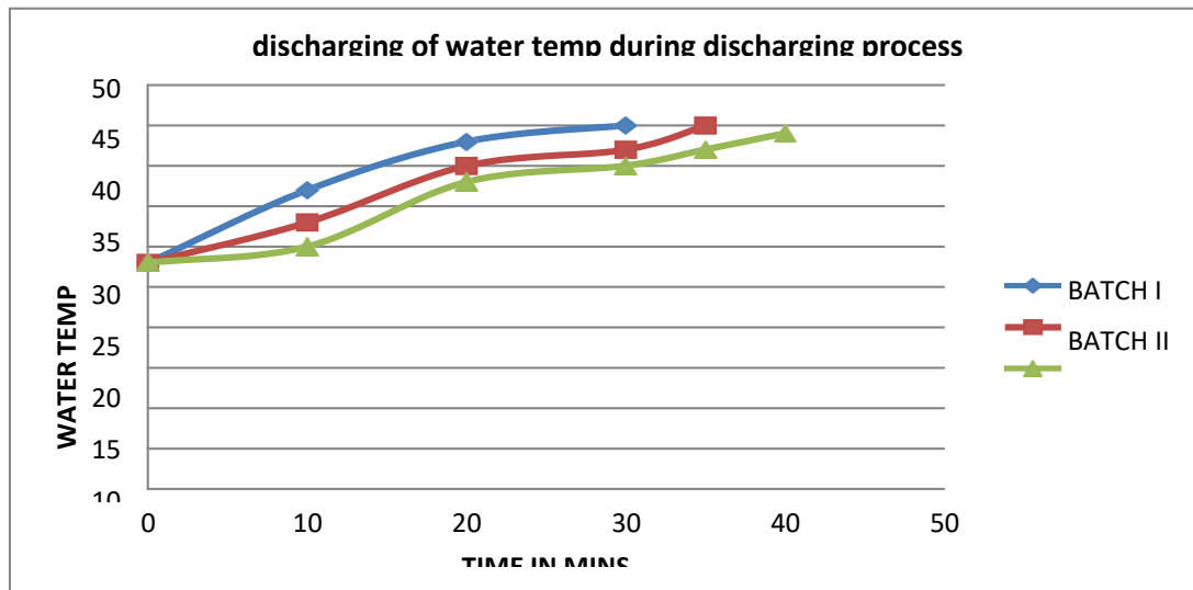
Fig 8: Discharging process
