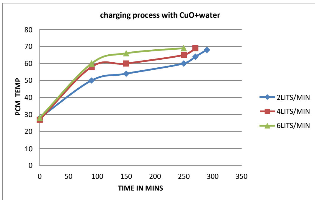
Fig 7: Charging process with CuO+HTF
