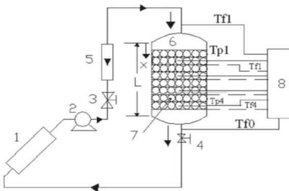
Fig 3: Schematic diagrammatic representation of Experimental Set-up
