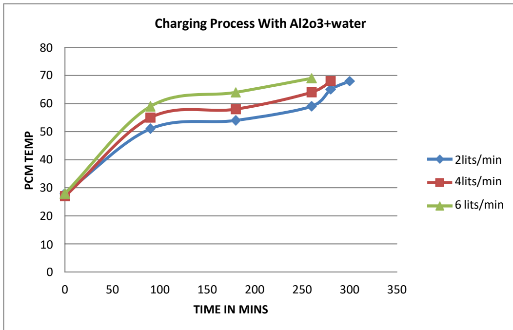
Fig 6: Charging process with Al 2 O 3 +HTF
