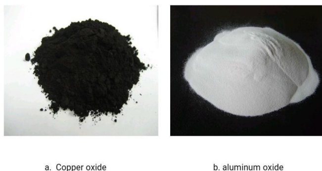
Fig 4: Nanoparticles
