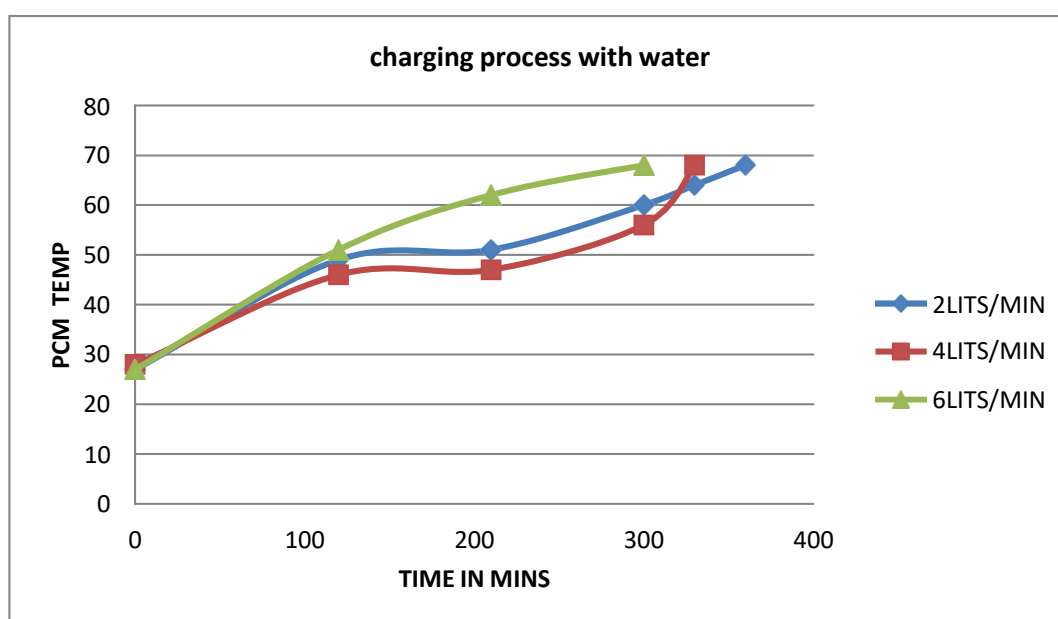
Fig 5: Charging process with HTF (water)
