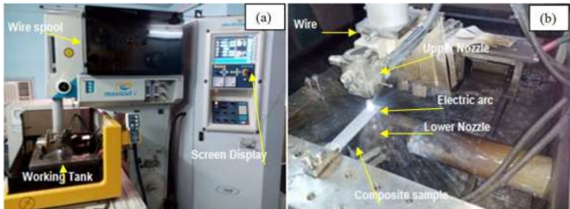
Figure 1(a) Wire EDM Machine and (b) Machining Zone
