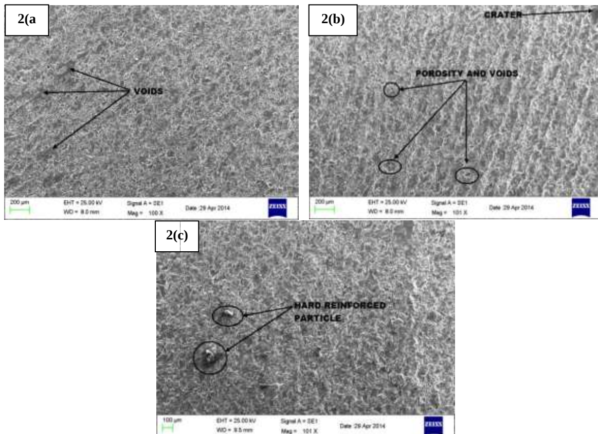
Figure 2 (a, b, c): Typical SEM Images of Machined Sample A359 +2% \text{Al}_2\text{O}_3 +2% \text{B}_4\text{C}
